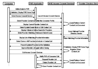
Figure 5: Provider Lists and Permissions (Diagram)
